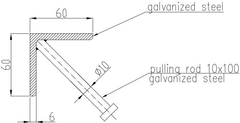
Angle 60x60x6 reinforced galvanized steel Section Scale 2:1
