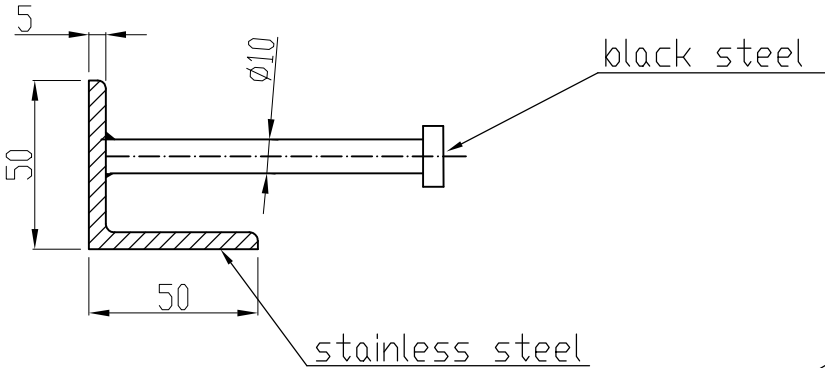
Angle 50x50x5 reinforced stainless steel Section Scale 2:1
