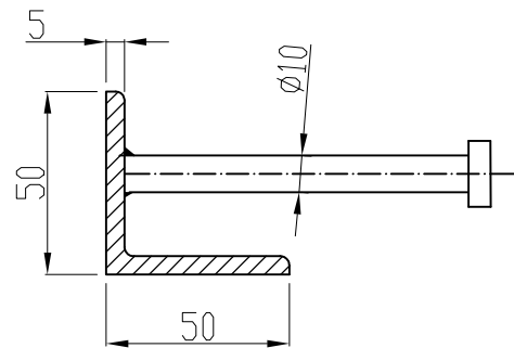
Angle 50x50x5 reinforced black steel Section Scale 2:1
