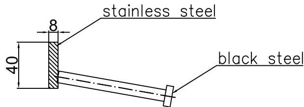
Conecto Single Strip Joint 08NA40 Section
