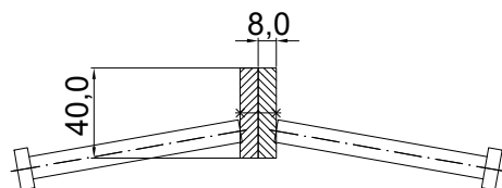
DOUBLE STRIP JOINT 08NA40 reinforced Section
