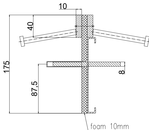
CONECTO DOWEL 10NA40-5D-T8 h=175 with foam 10mm Section Scale 2:1
