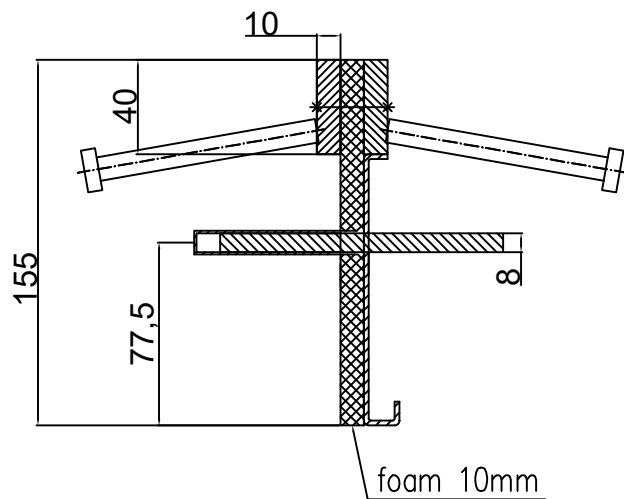
CONECTO DOWEL 10NA40-5D-T8 h=155 with foam 10mm Section Scale 2:1
