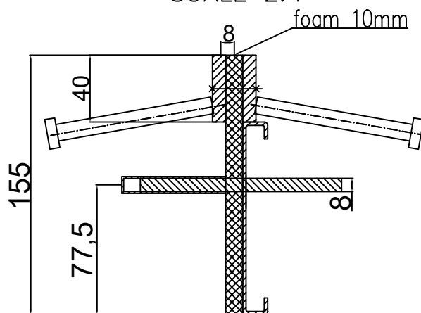
Conecto Dowel 08NA40-5D-T8 h=155 with foam 10mm SECTION SCALE 2:1
